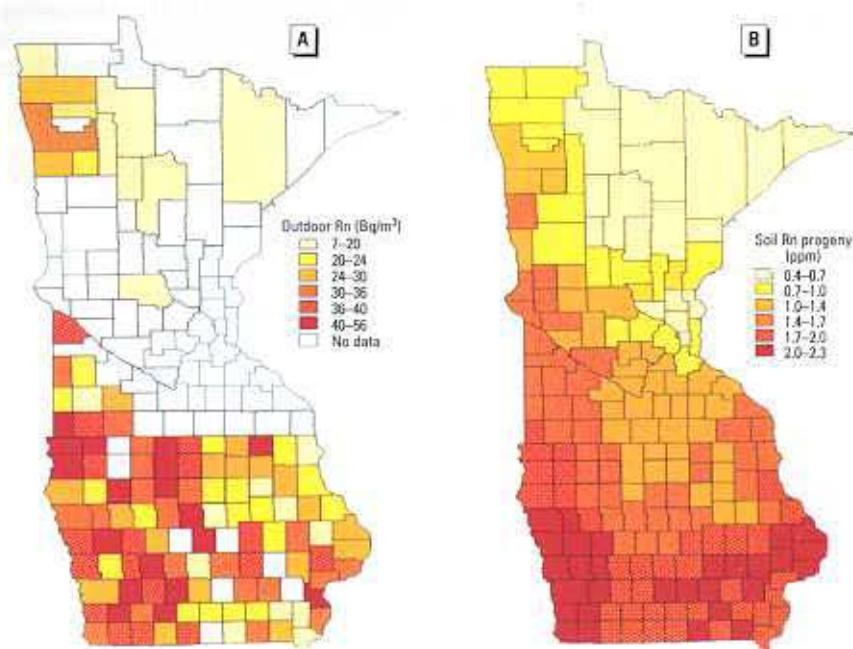
Figure 4. (A) County-average outdoor radon concentrations and (B) radon progeny in the surface soil estimated from National Uranium Resource Evaluation data (29). White areas show counties where no radon measurements were made.
