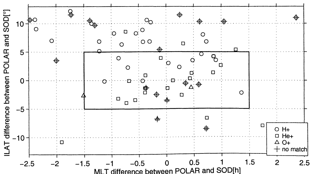
Figure 6. The scatterplot of Polar events in \Delta\text{MLT}-\Delta\text{ILAT} plane, where \Delta\text{MLT} and \Delta\text{ILAT} are the corresponding differences between Polar and SOD during wave observation.
