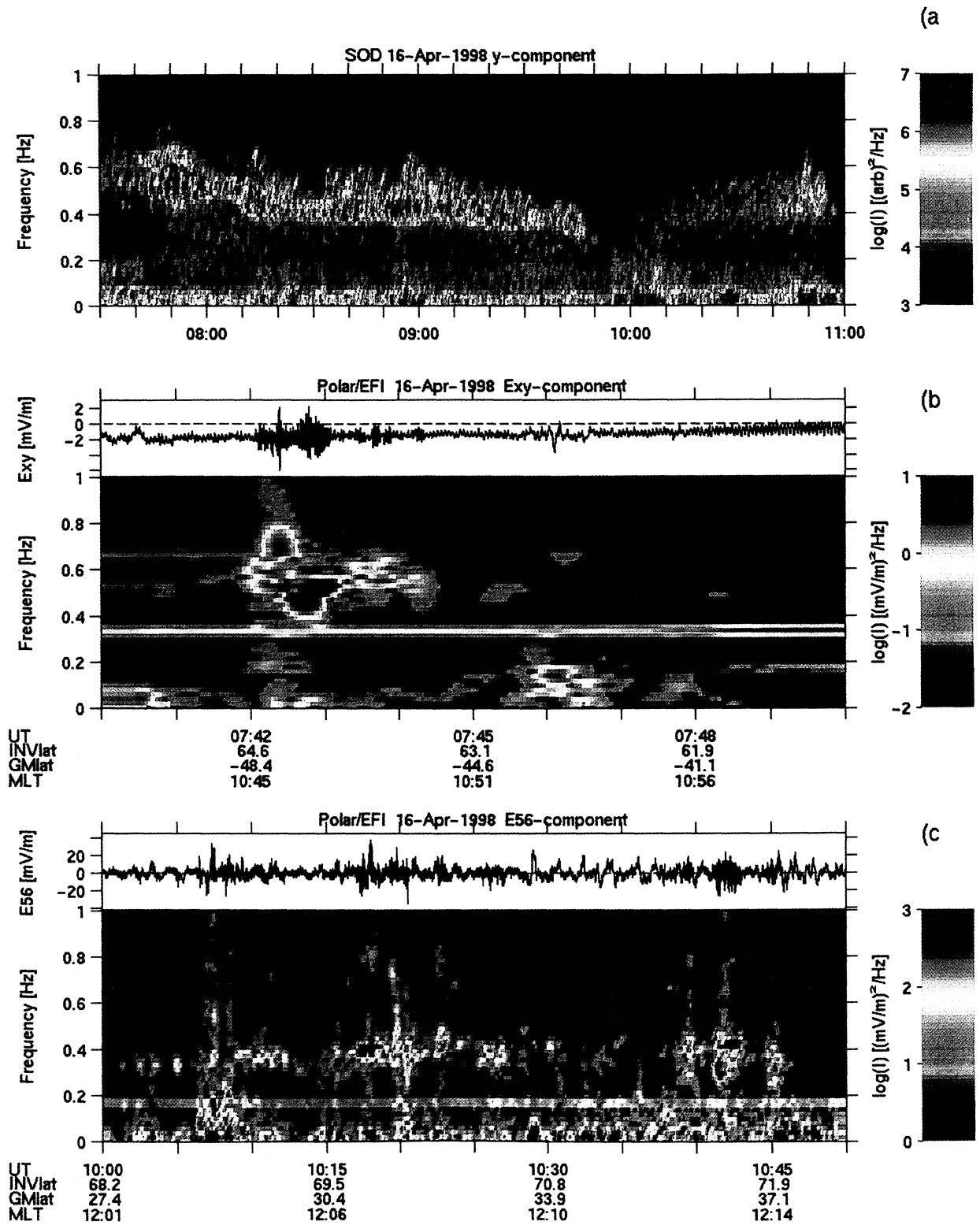
Plate 1. April 16, 1998, sample event. (a) Pc1 pulsation activity at Sodankylä (SOD) at 0730–1100 UT. (b) Electromagnetic ion cyclotron (EMIC) observations by Polar at 0740–0750 UT. (c) EMIC observations by Polar at 1000–1100 UT.
